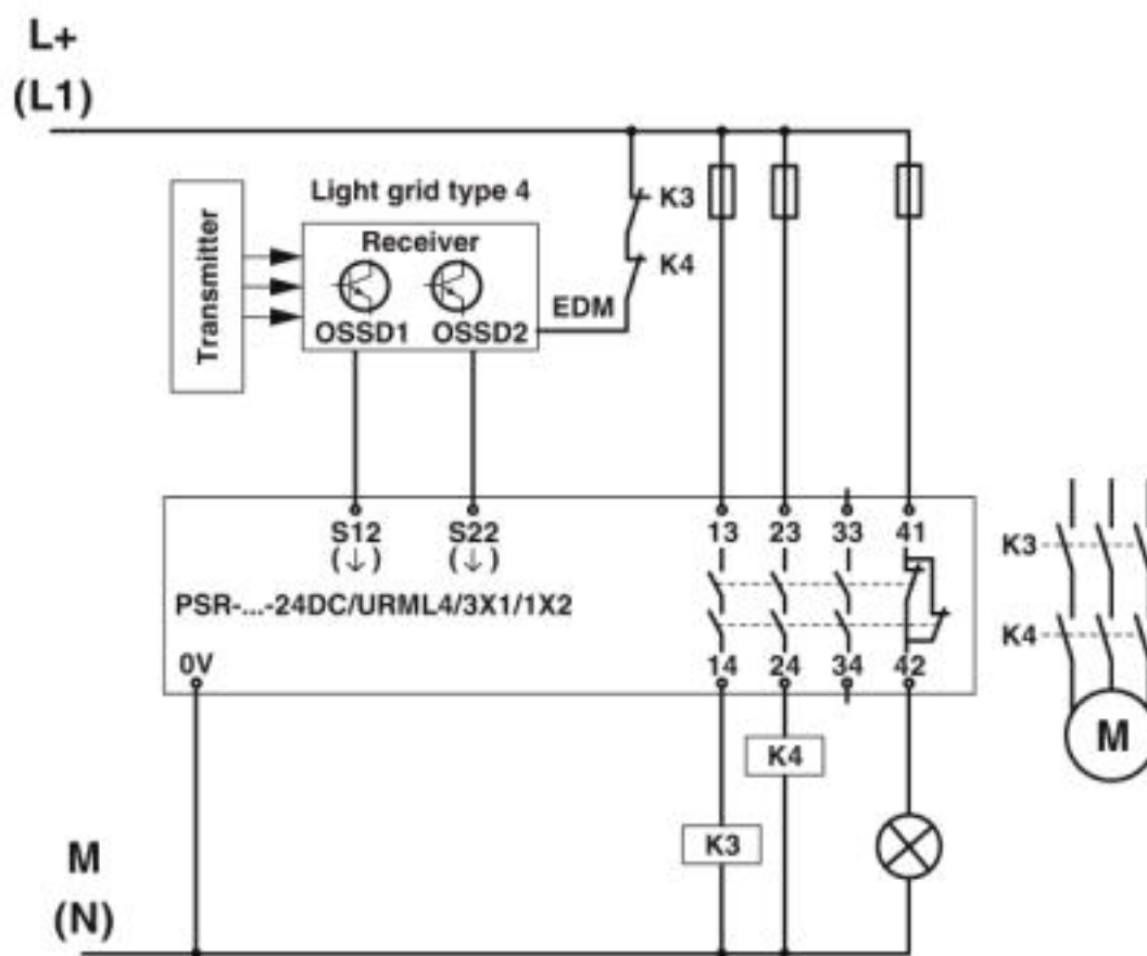
Application drawing
