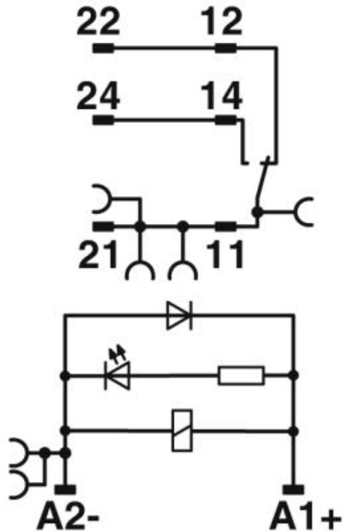
Circuit diagram
