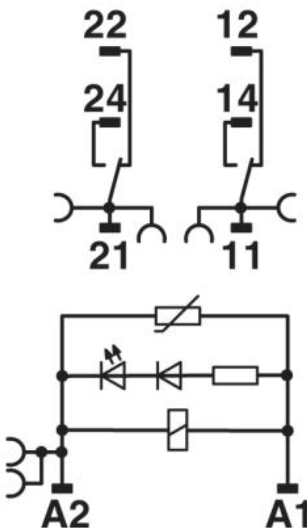
Circuit diagram
