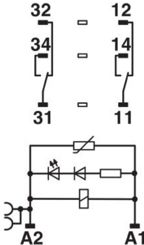
Circuit diagram
