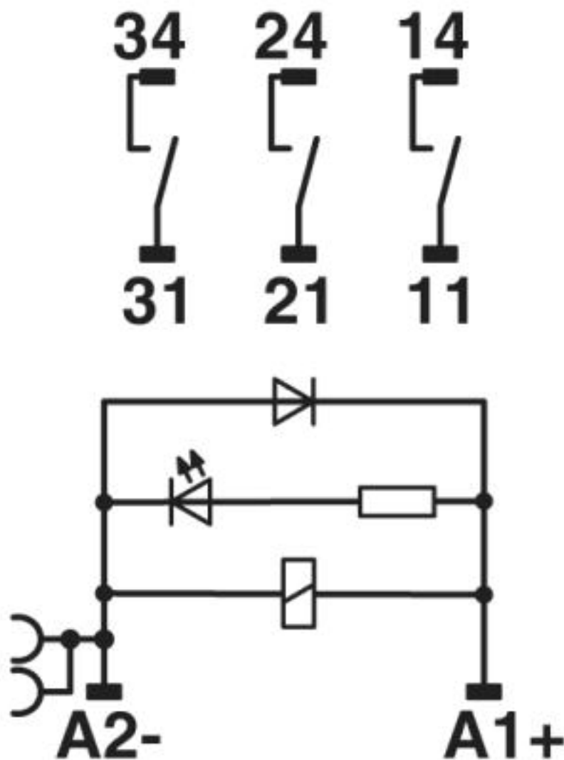
Circuit diagram
