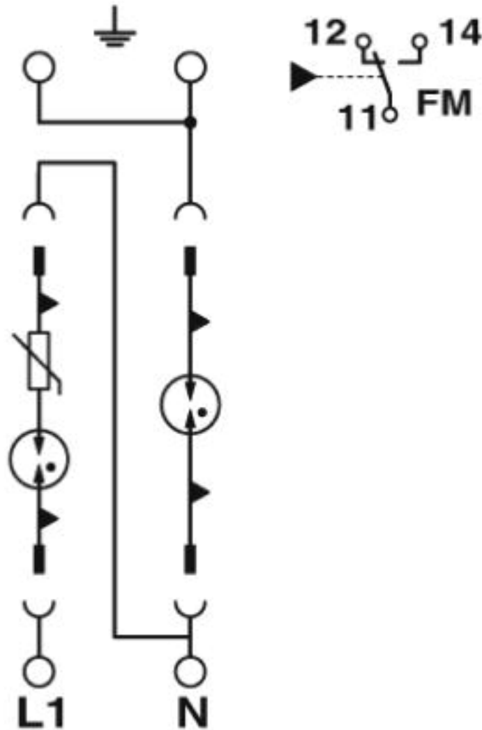
Circuit diagram
