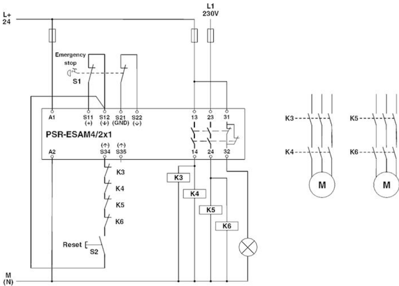
Circuit diagram
