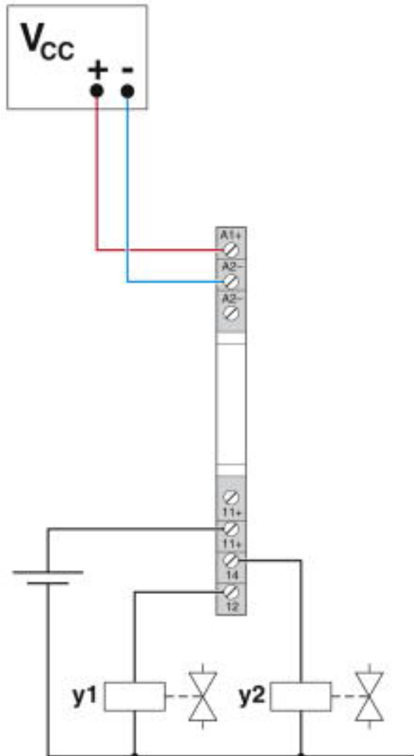
Application drawing
