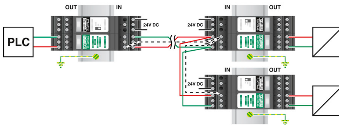
Application drawing
