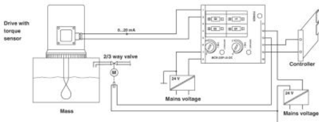
Application drawing
