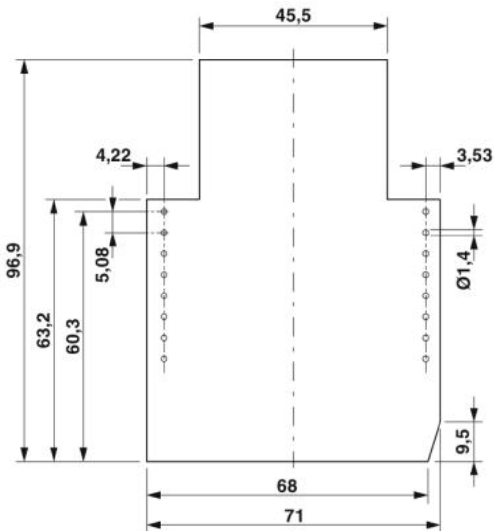
Dimensional drawing
