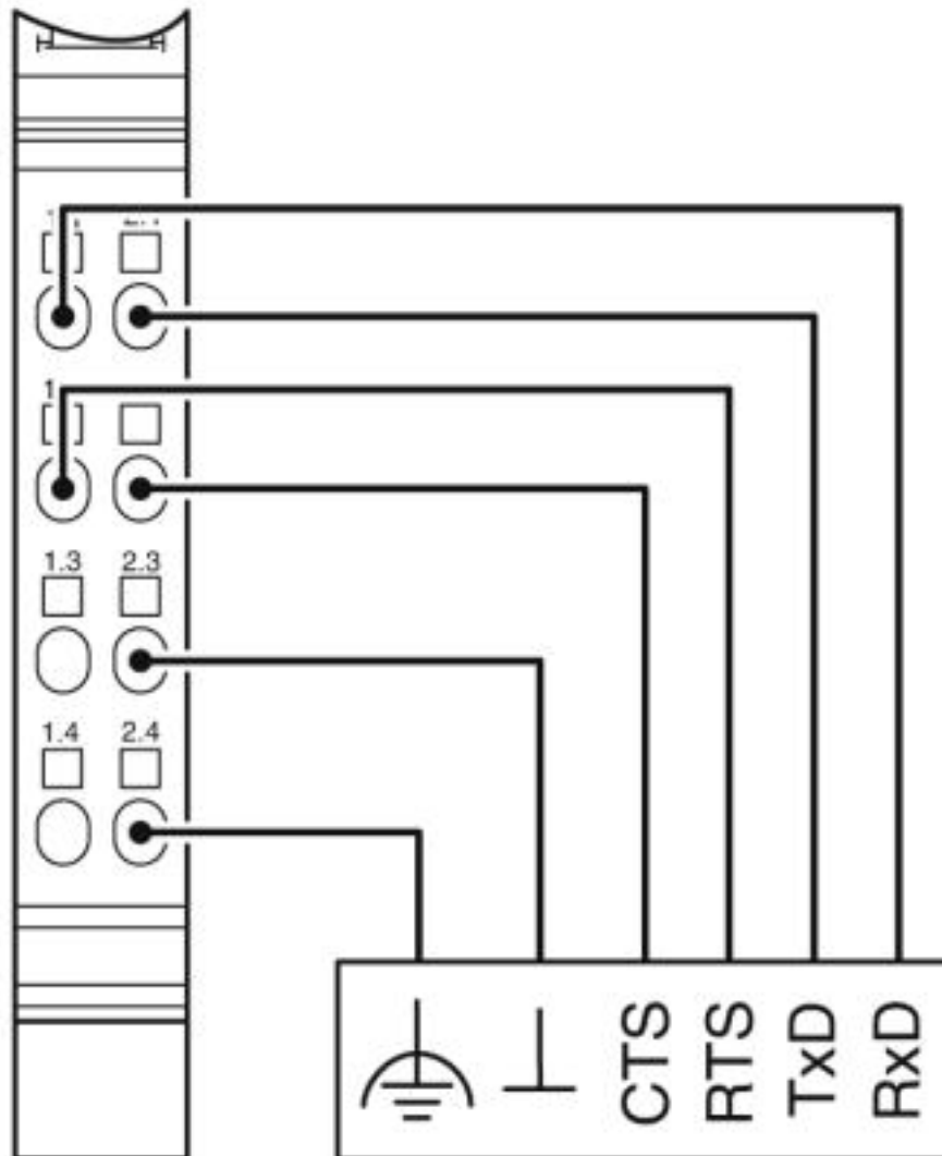
Connection diagram
