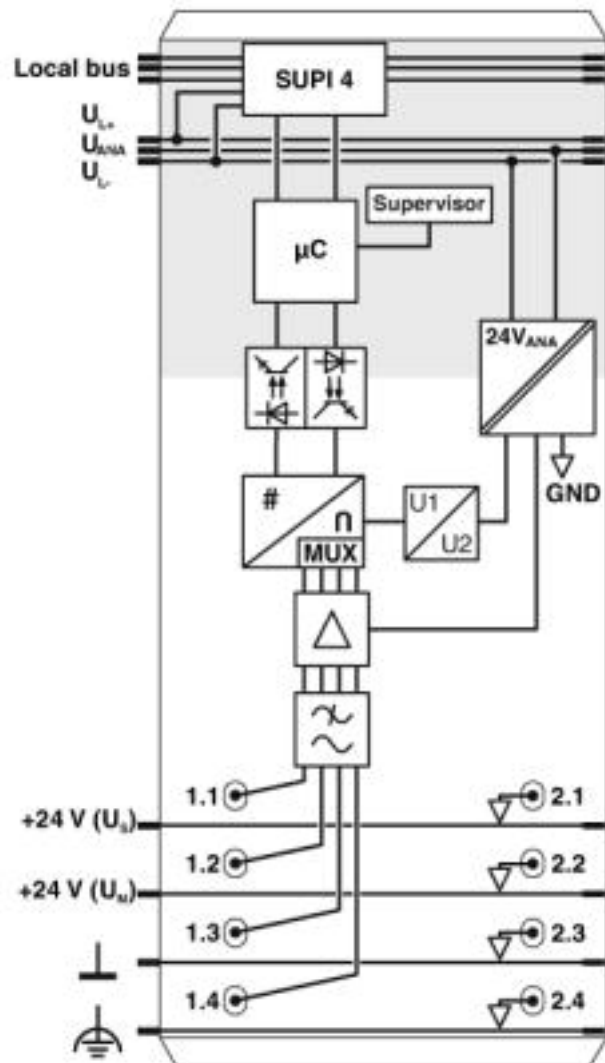
Block diagram
