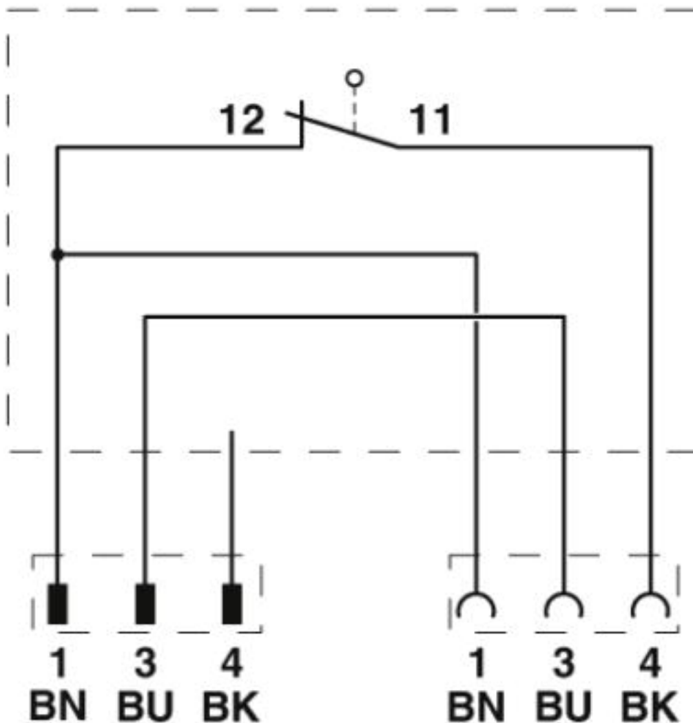
Circuit diagram
