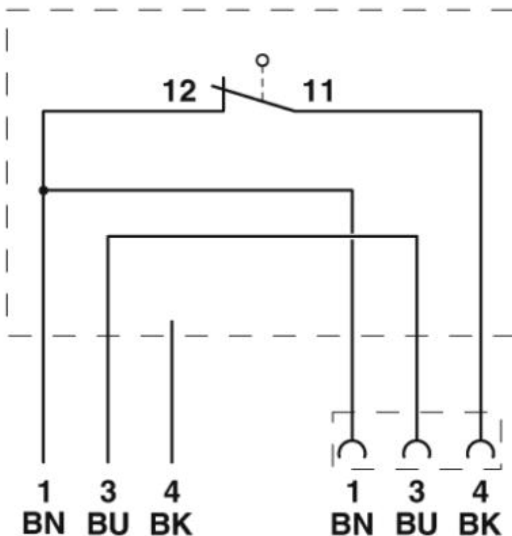
Circuit diagram
