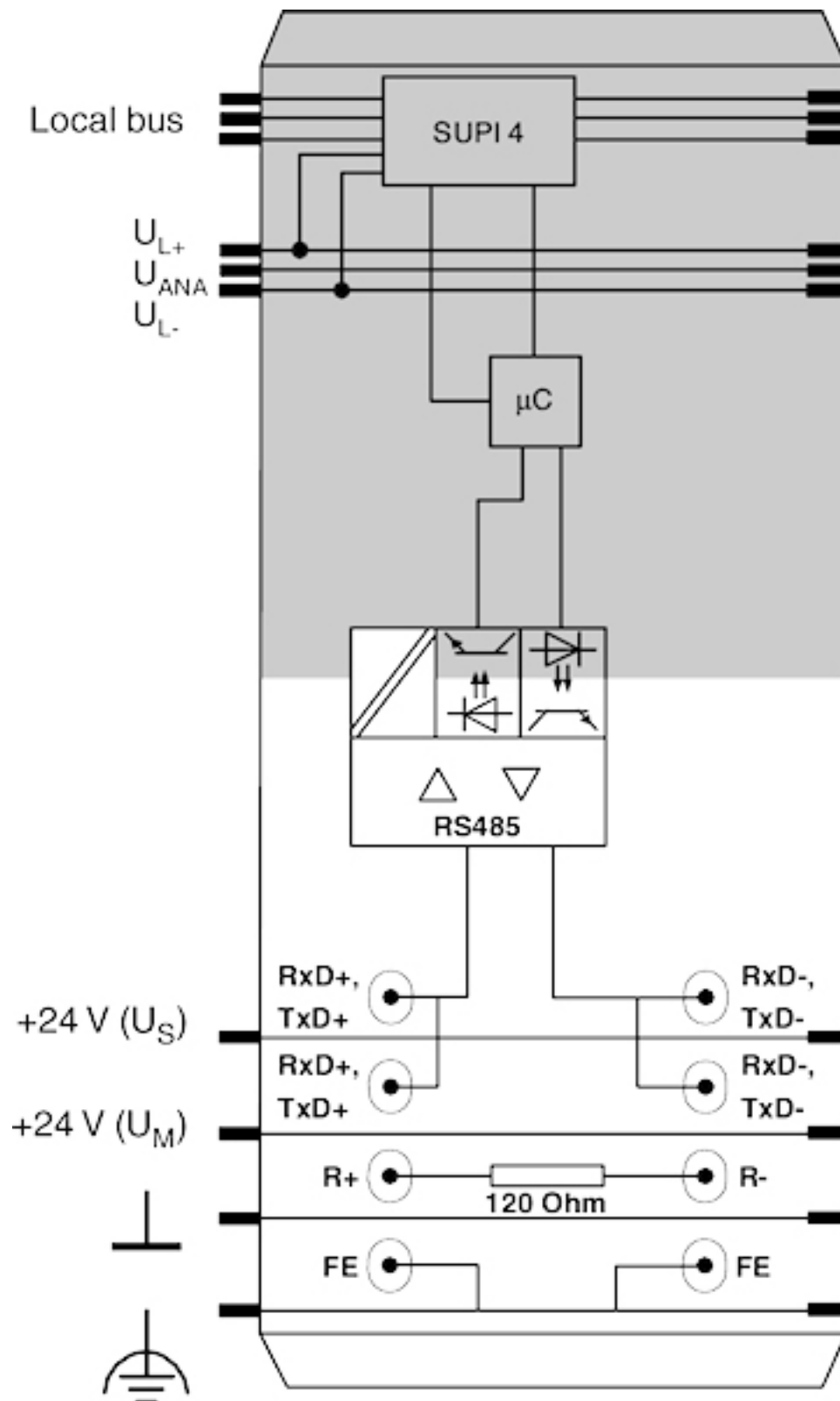
Block diagram
