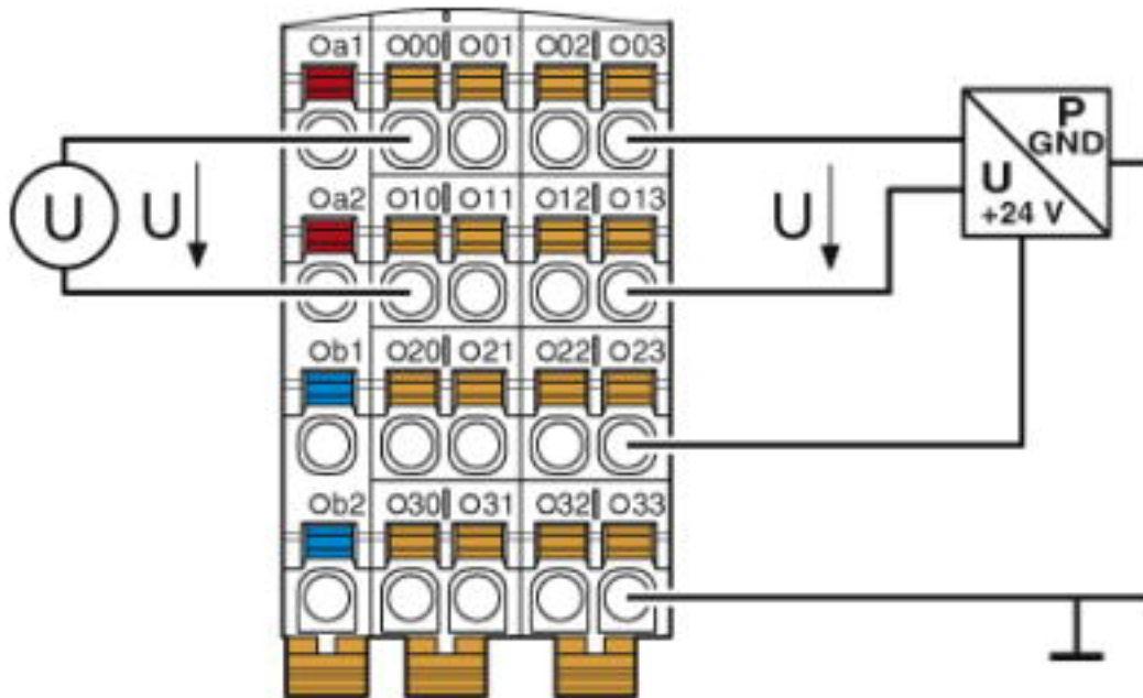
Connection diagram
