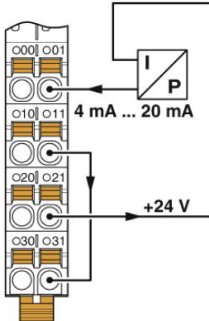
Connection diagram
