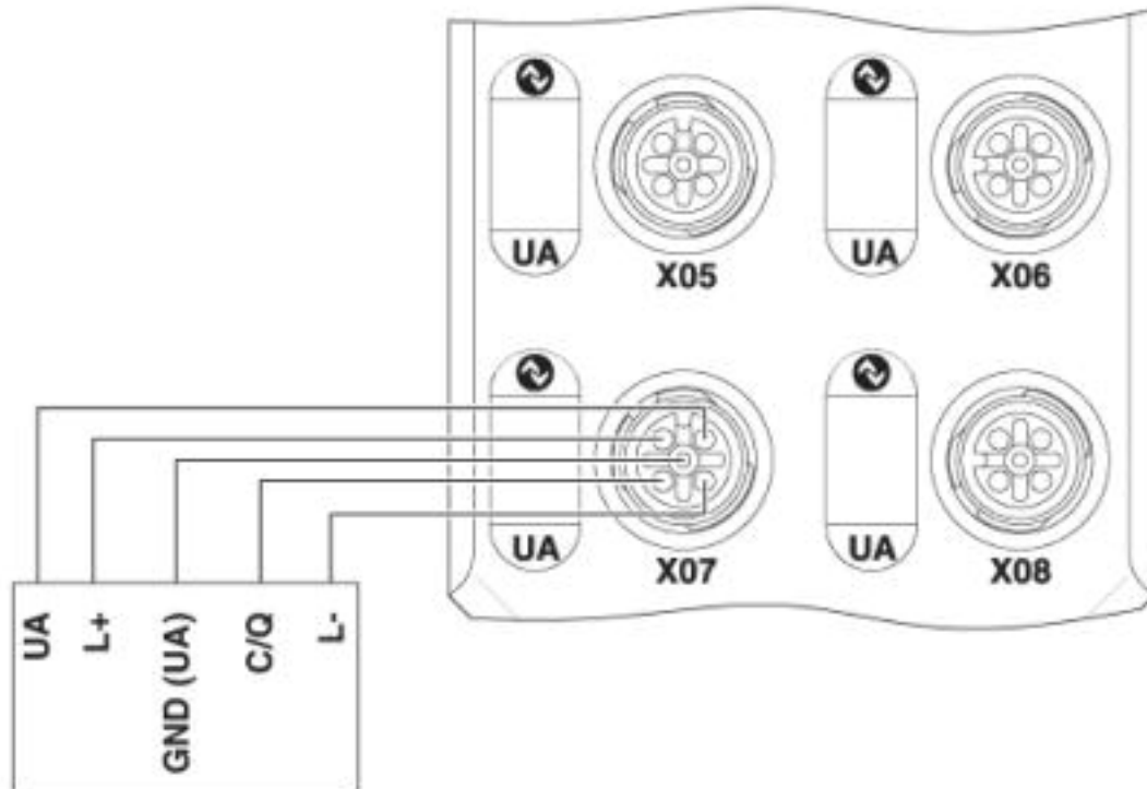
Connection diagram
