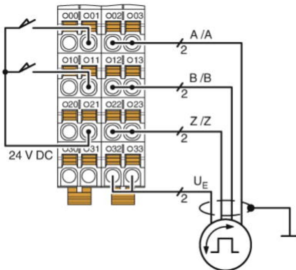
Connection diagram
