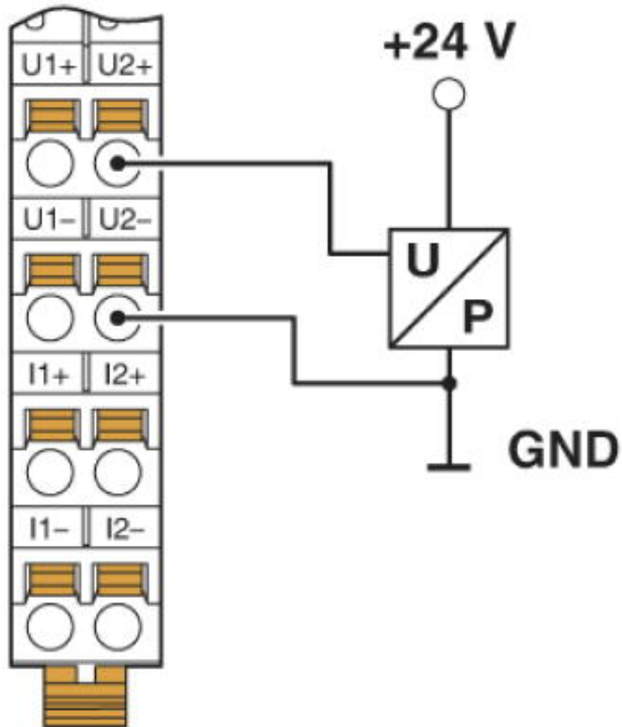
Connection diagram
