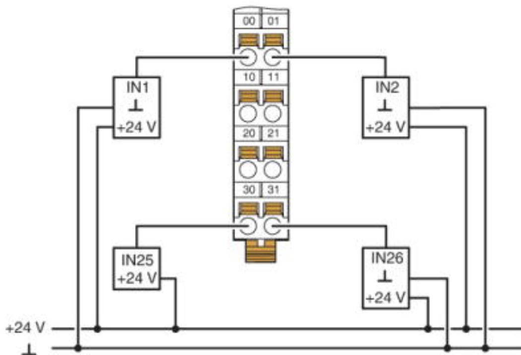
Connection diagram
