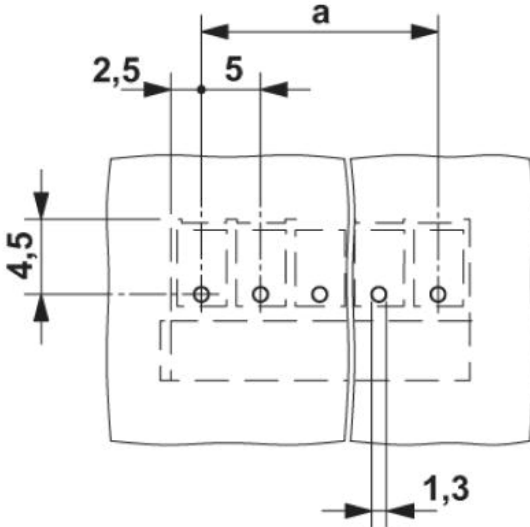
Drilling diagram
