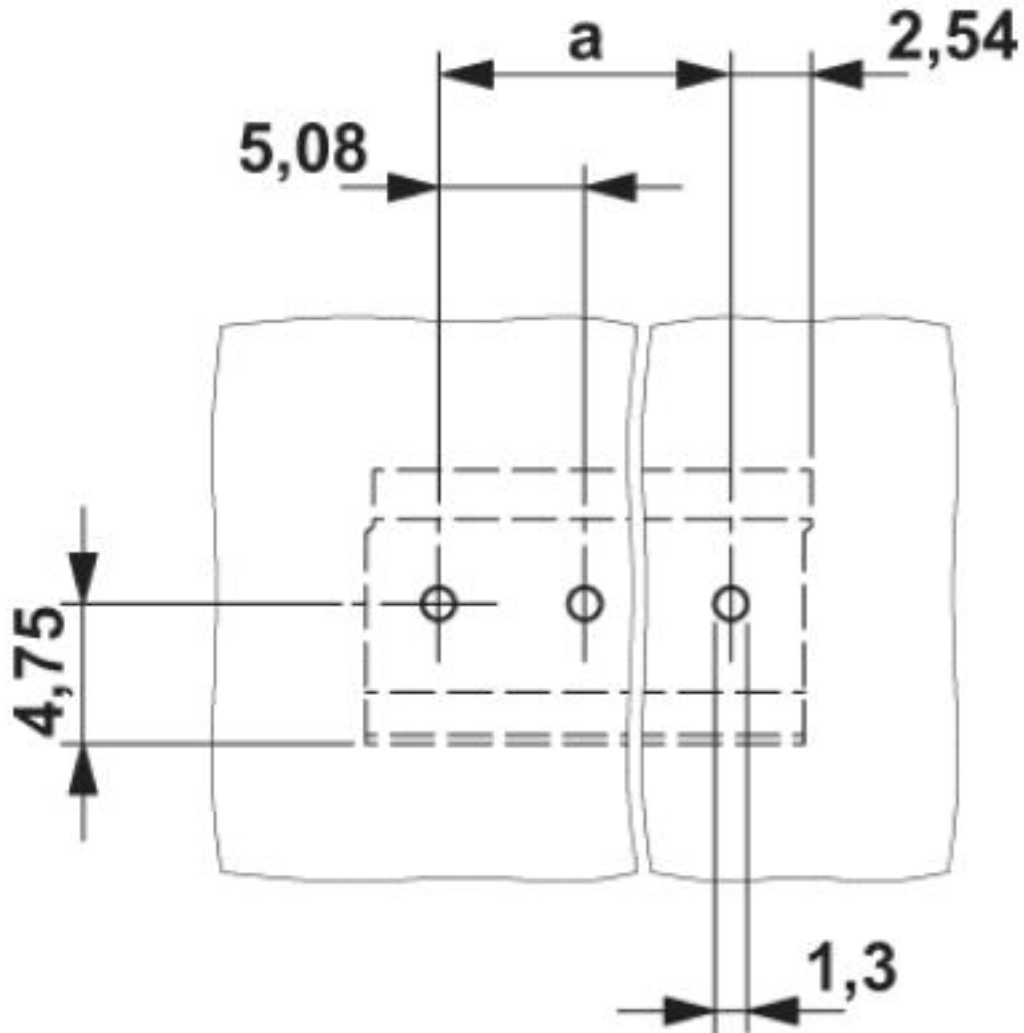
Drilling diagram
