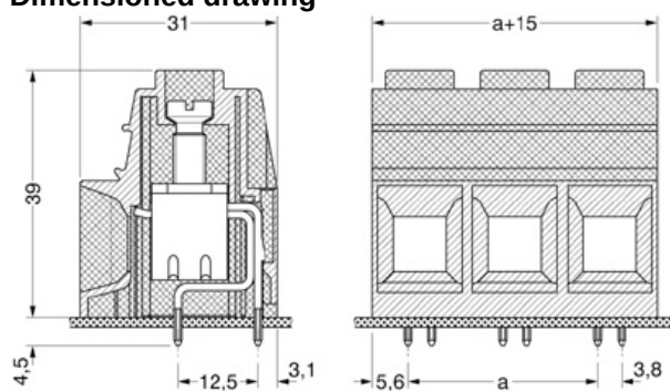
Dimensioned drawing
