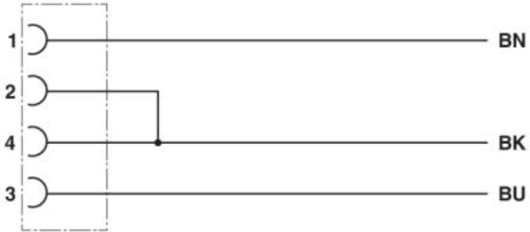
Contact assignment of M12 sockets bridged
