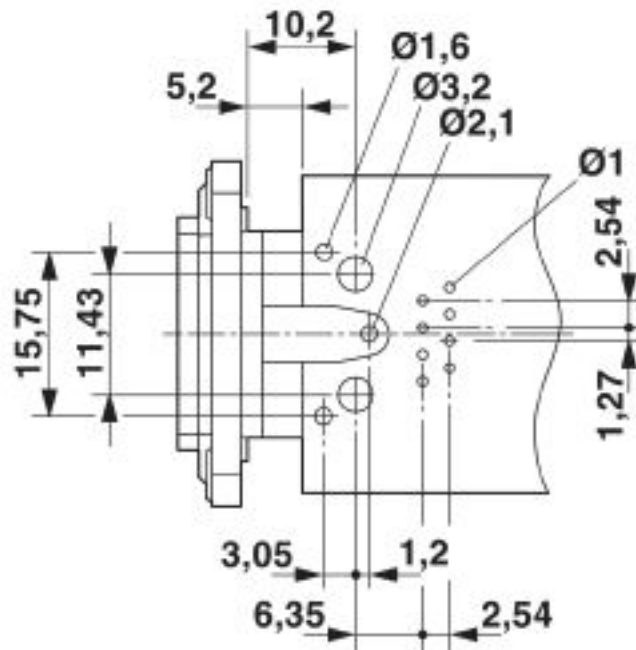
Drilling diagram
