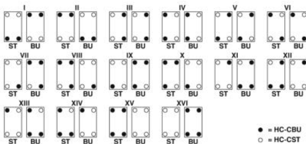
Schematic diagram
