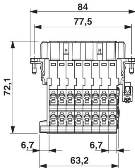
Dimensional drawing
