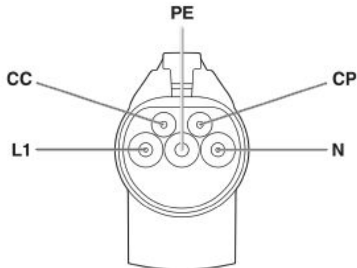
Connection diagram
