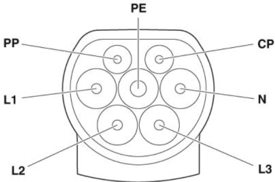
Connection diagram
