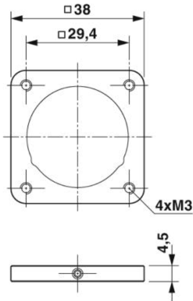
Dimensional drawing
