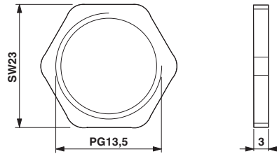
Dimensional drawing
