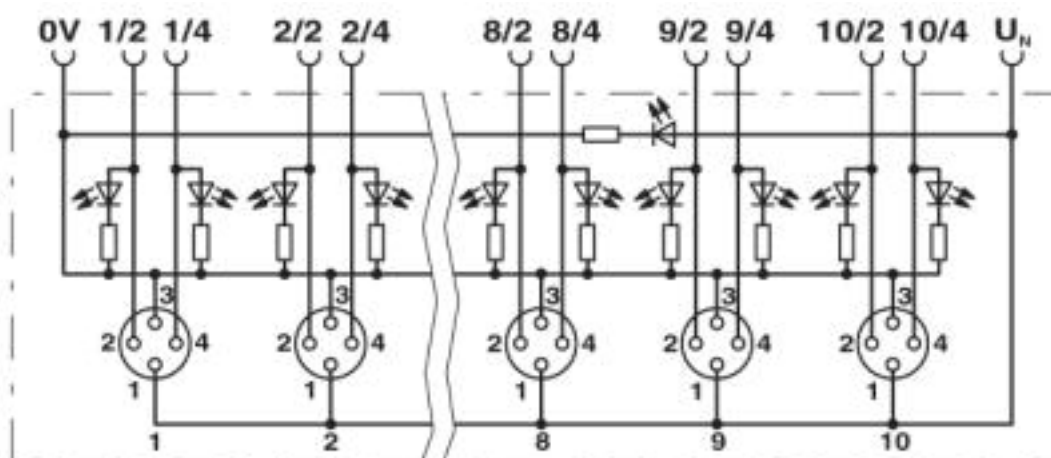
Circuit diagram
