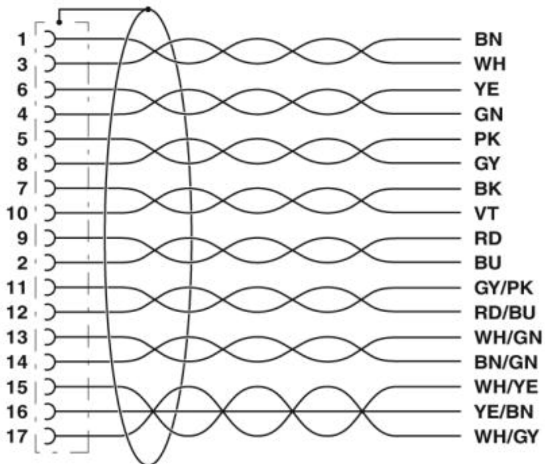
Circuit diagram
