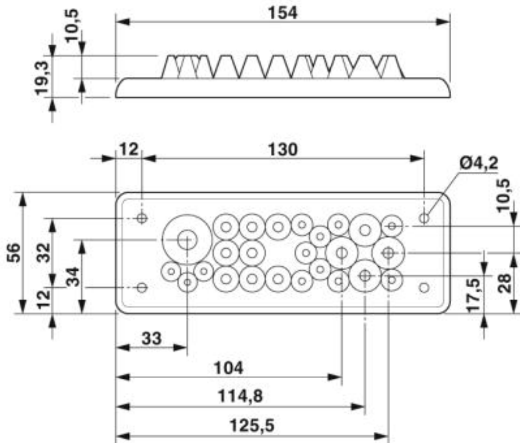
Dimensional drawing
