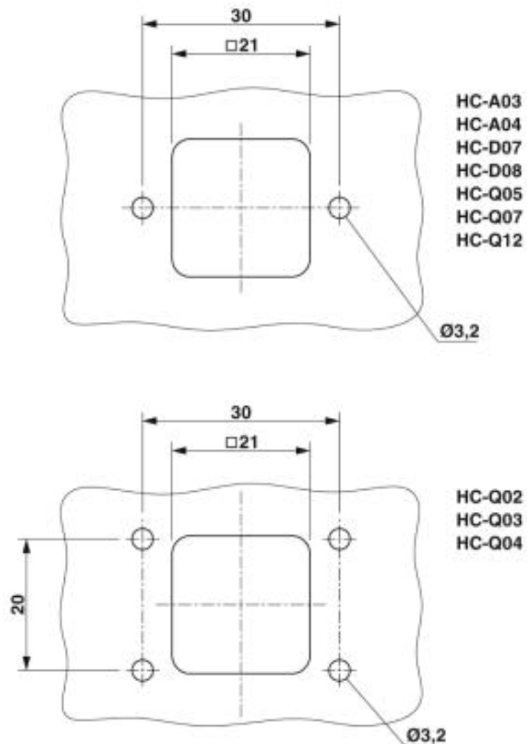
Dimensional drawing
