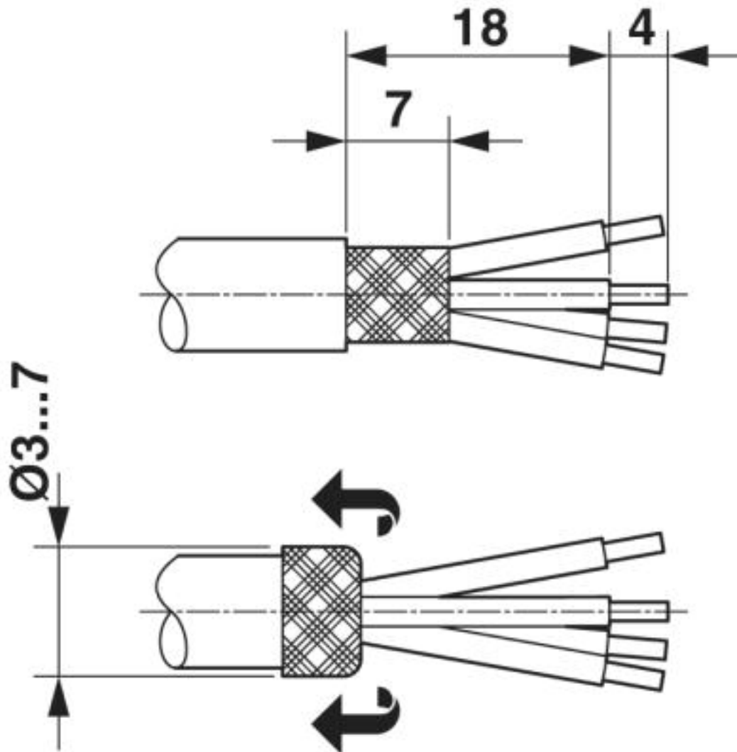
Dimensional drawing
