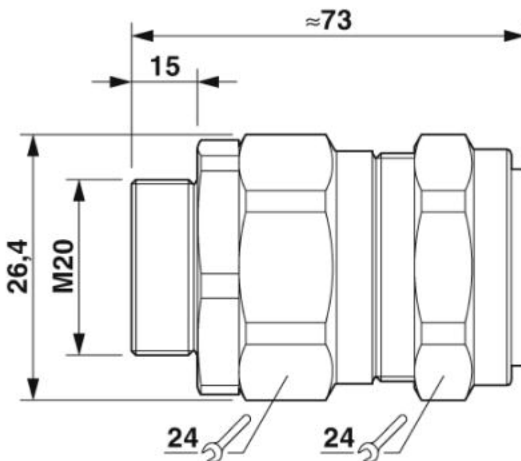
Dimensional drawing
