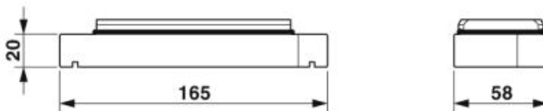
Dimensional drawing
