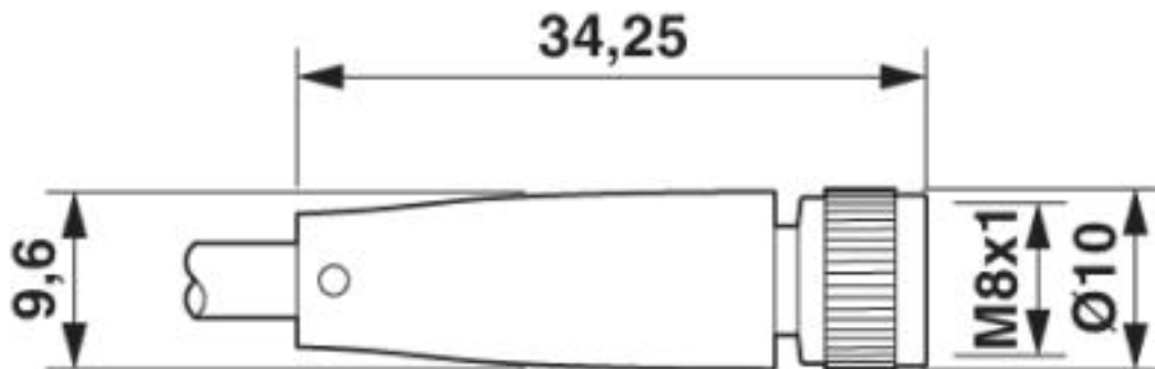
Dimensional drawing
