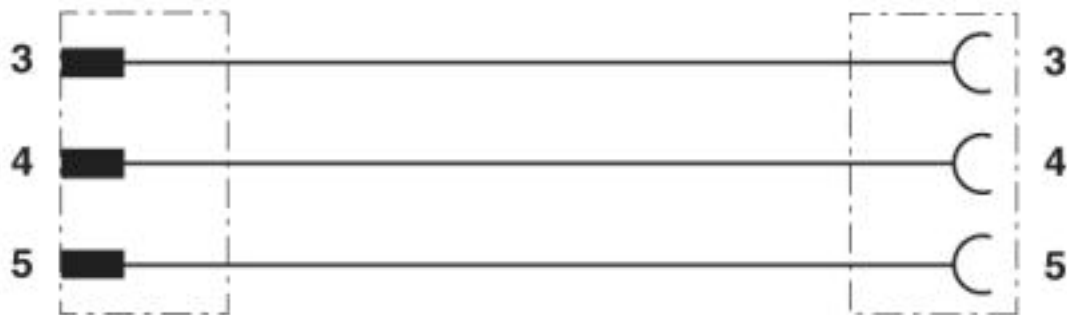
Contact assignment of the M12 connector and the M12 socket
