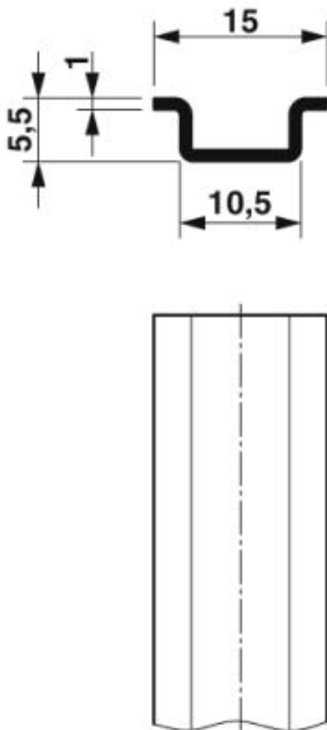
Dimensional drawing
