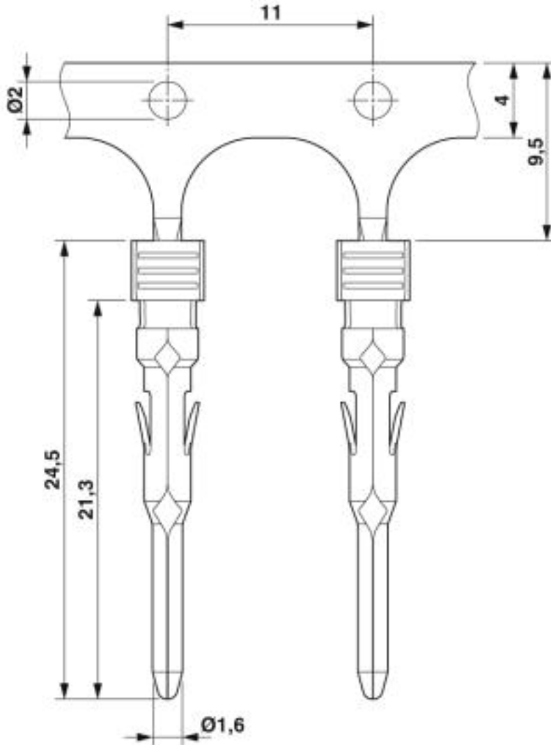
Dimensional drawing
