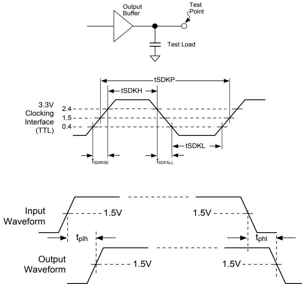
Figure 1. Clock Waveforms
