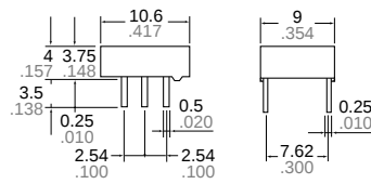
External dimensions Standard PC board terminal
