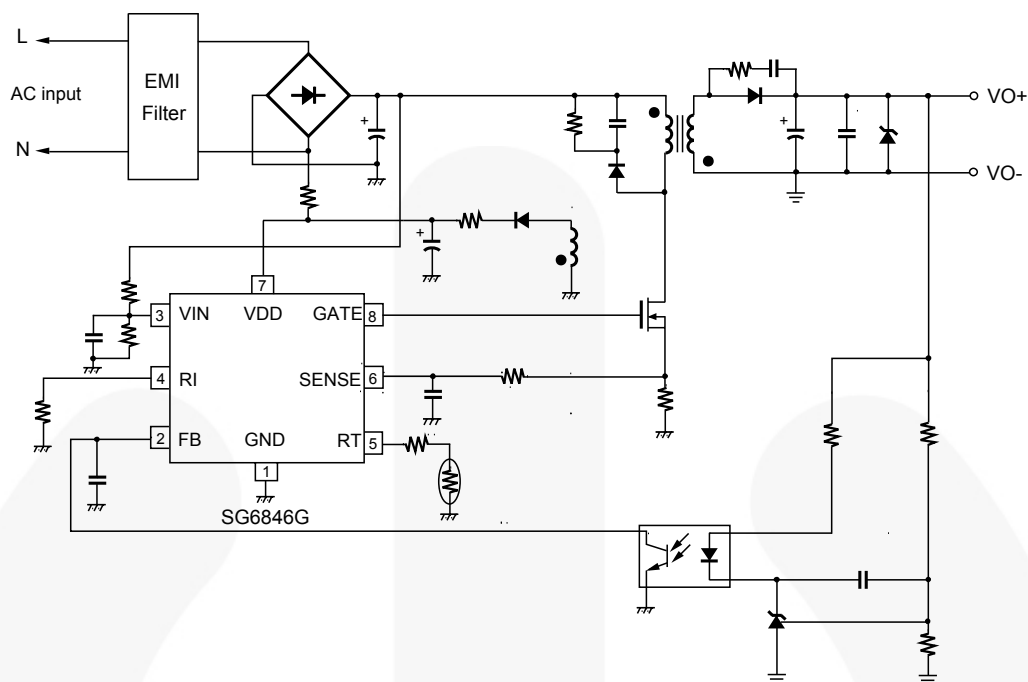
Figure 1. Typical Application
