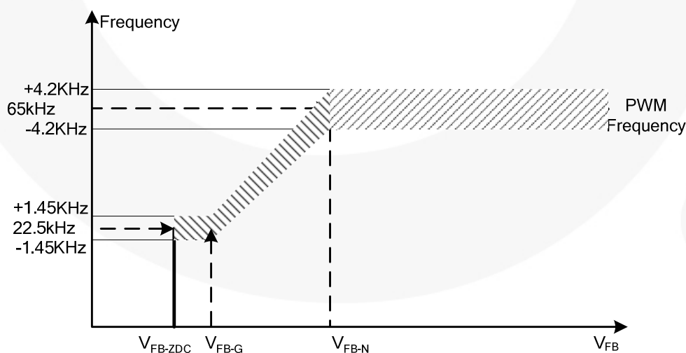
Figure 5. PWM Frequency
