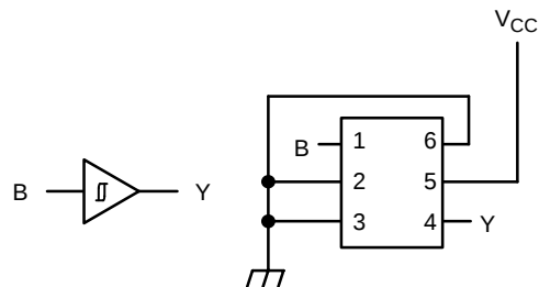
Figure 8. Buffer (When A = C = "L")
