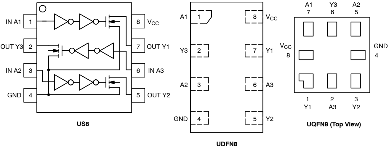
Figure 2. Pinout
