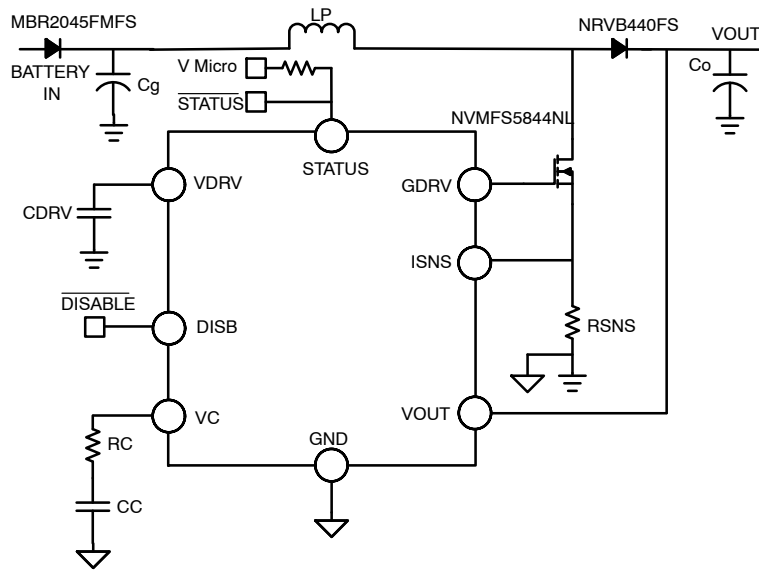
Figure 1. Typical Application
